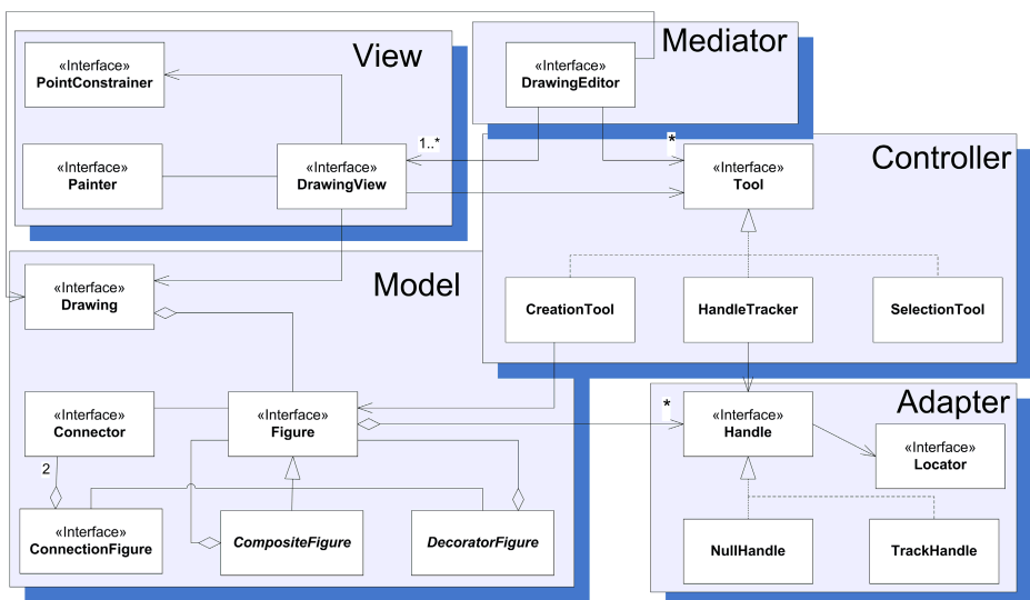
Fig. 4. Classification of abstractions
