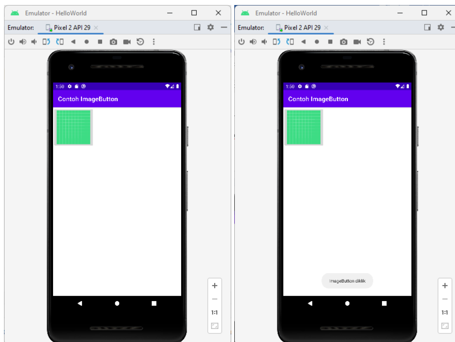
Gambar 4.12 Contoh ImageButton
